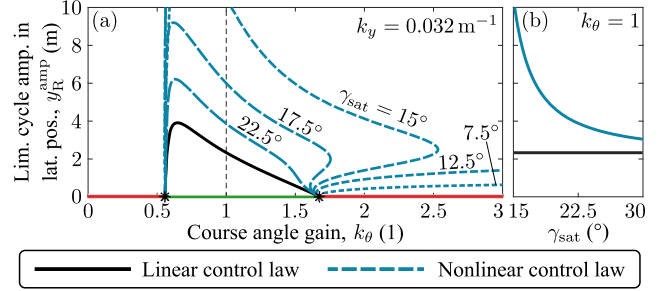
Fig. 7. (a) Bifurcation diagram using the linear (black) and the nonlinear (blue) control law with different saturation levels \gamma_{\text{sat}} . (b) Limit cycle amplitude as a function of the saturation parameter \gamma_{\text{sat}} .
