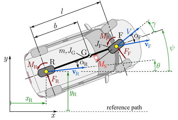
Fig. 1. Bicycle model with steering dynamics.
