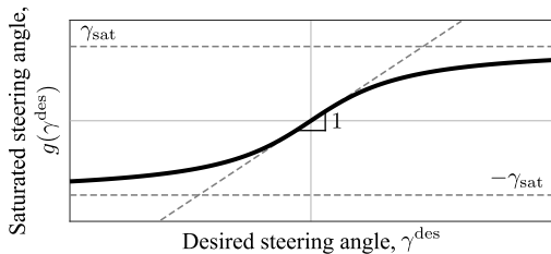
Fig. 6. The continuous wrapper function g(\gamma^{\text{des}}) in (18).
